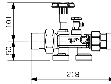
Module By-pass 5/4" Ech:1/5
